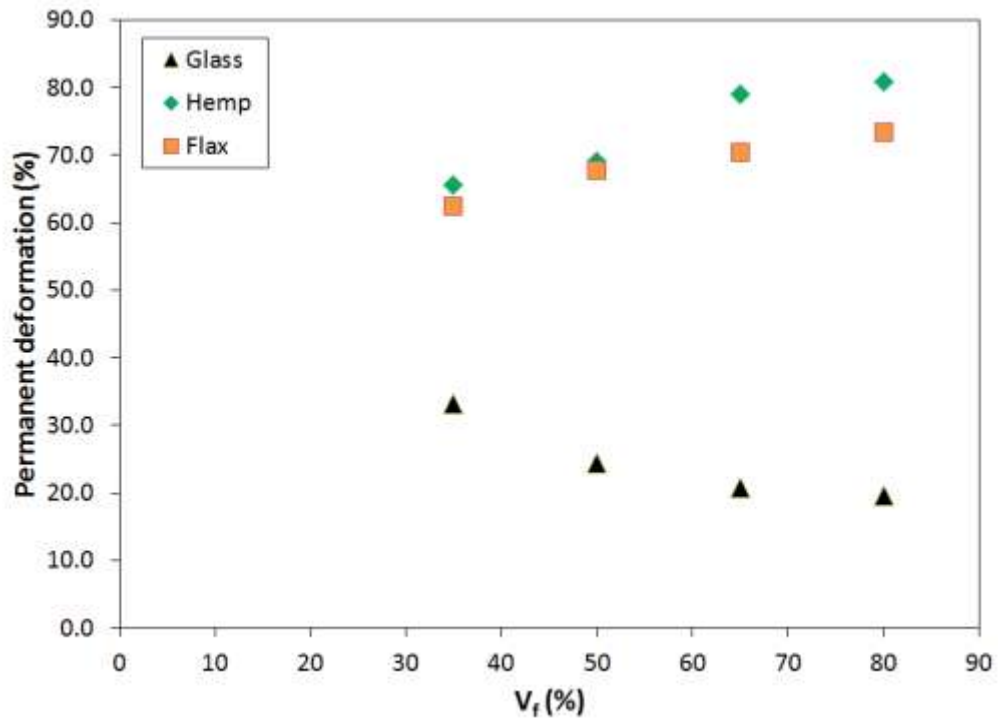
Figure 2: Evolution of the permanent deformation with fibre volume fraction. The results were very reproducible with less than 3% of standard deviation measured for each reinforcement
